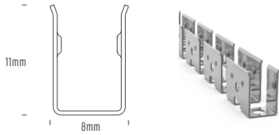
AQS-402-ACC-02 Bendable S Channel
