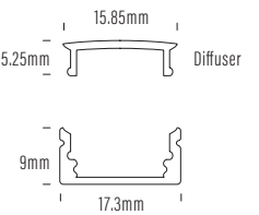
AQS-100-AL-02-2M Aluminium Profile PMMA Diffuser
