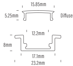
AQS-100-AL-001-2.5M-SC Aluminium Profile PMMA Diffuser
