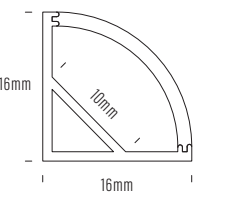
AQS-100-AL-003-2.5M-A1 Aluminium Profile Corner Recess with Opal PC Cover
