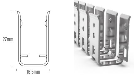
AQS-500-ACC-AL4-01 Bendable S Channel Note: Compatible with AQS-420
