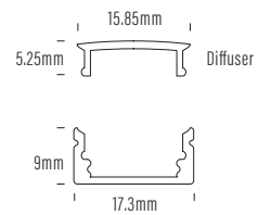
AQS-100-AL-02-1M Aluminium Profile PMMA Diffuser
