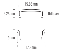
AQS-100-AL-02-2.5M Aluminium Profile PMMA Diffuser
