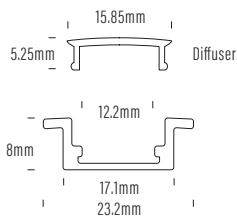
AQS-100-AL-001-2.5M-WH Aluminium Profile PMMA Diffuser
