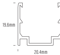
AQS-510-ACC-AL-02 2m Aluminium
