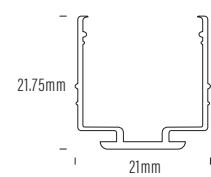
AQS-510-ACC-AL2-02 2m Aluminium
