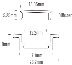
AQS-100-AL-001-2.5M-BK Aluminium Profile PMMA Diffuser
