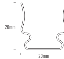
AQS-510-ACC-01-SS 316SS Mounting Clip
